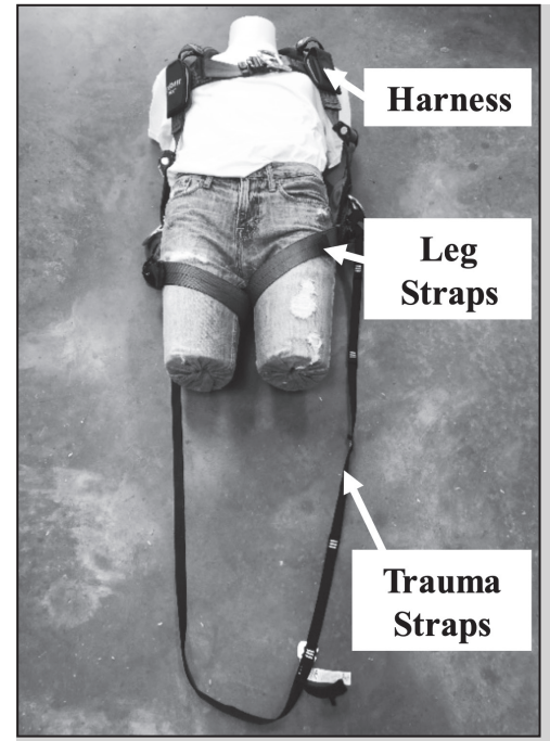
Figure 1: Harness with suspension trauma straps.
