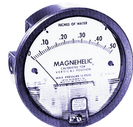
A portable pressure gauge can test static pressure difference between inside and outside of a house.
