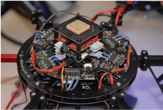
Miniaturization of electronics makes sUAS possible.
