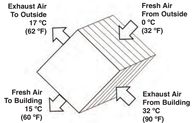
Figure 2. A cross-flow heat recovery ventilator (with typical temperatures). Arrows indicate the directions of airflows.
