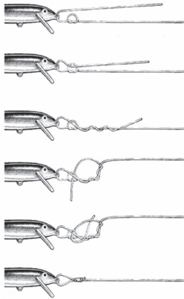
Rapala Knot
