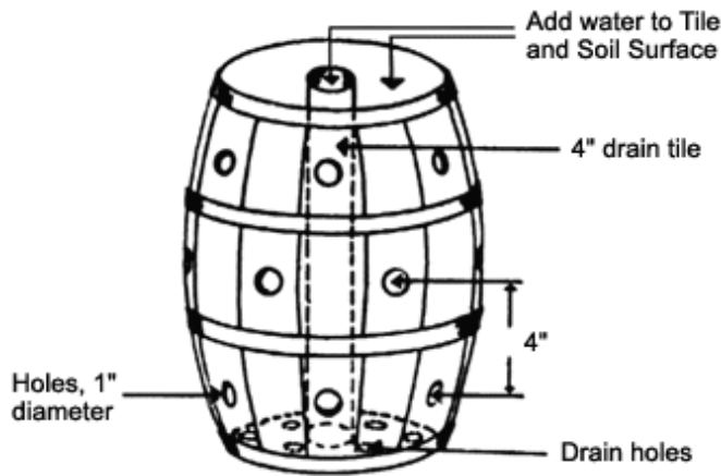
Figure 3 A Barrel Planter
