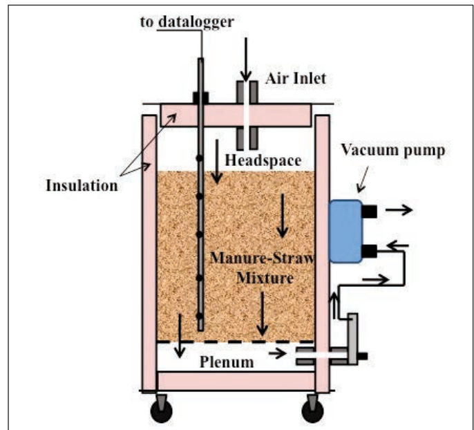
Figure 2. Biodrying unit.
