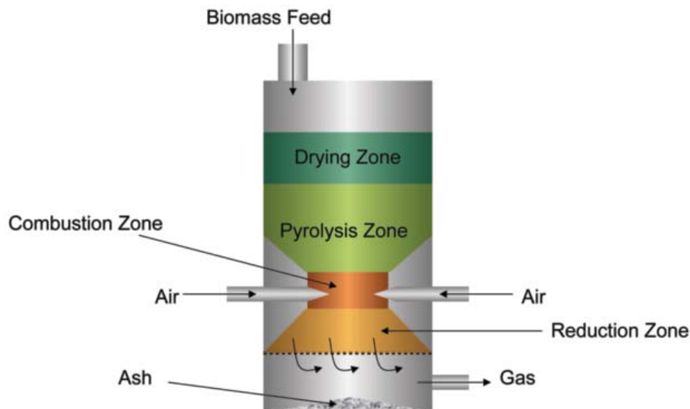
Figure 2. Downdraft fixed bed gasifier (Source: G. Foley and G. Barnard. 1985. Biomass Gasification in Developing Countries. Earthscan, London, UK)
