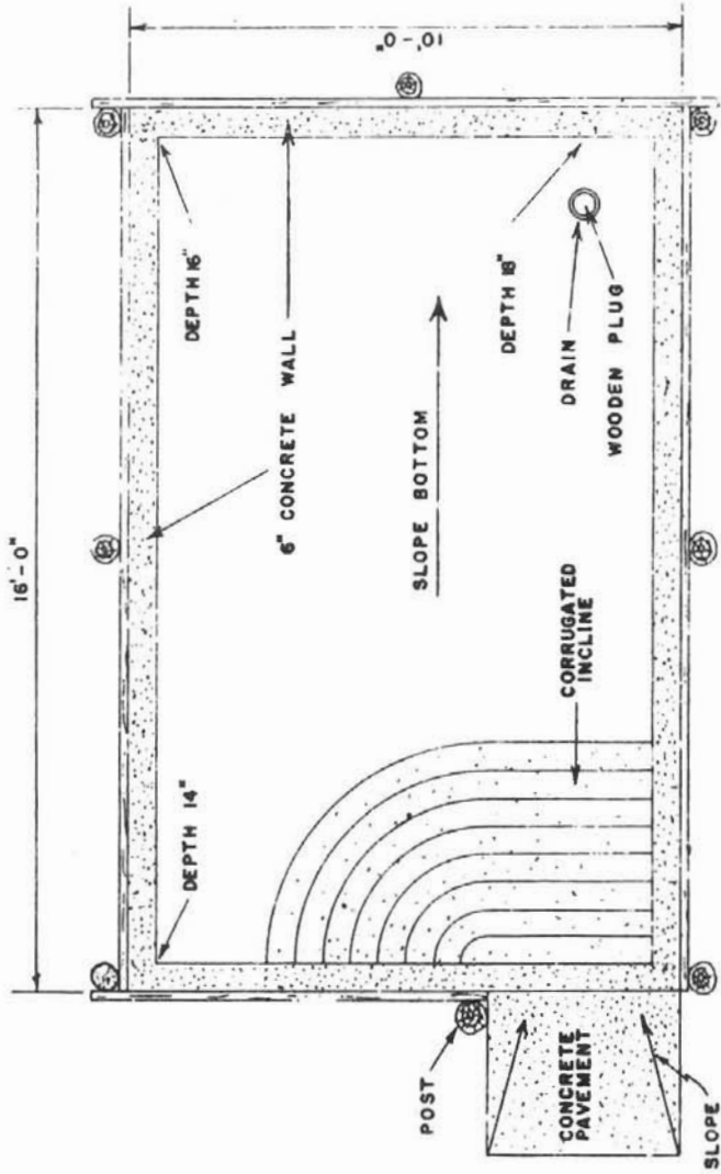
FLOOR PLAN
