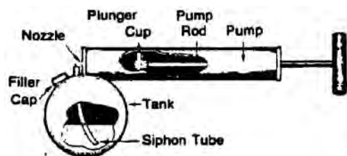
Figure 27. Flit Gun Sprayer.
