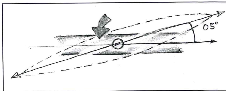
FIGURE 11.2A. Flat fan nozzles should be angled at approximately 5° from parallel to the boom. All nozzles should be turned the same direction. Graphics by Will Hampton.
