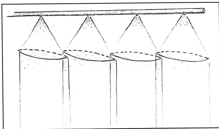
FIGURE 11.2B. Angling nozzles assures a similar deposition of spray material all along the spray band, without the particles shearing and drift potential seen when the edges of spray patterns collide in the air. Graphics by Will Hampton.
