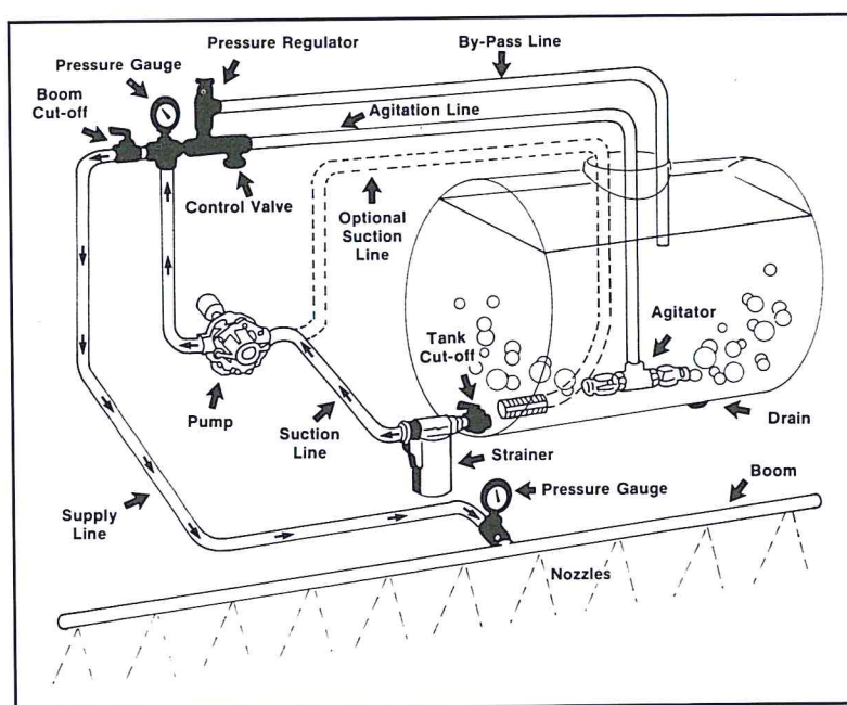
FIGURE 11.1. Components of a properly designed weed control sprayer.
