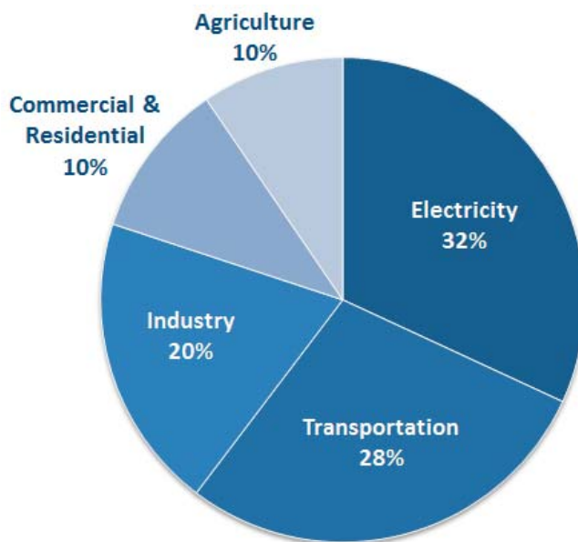
Figure 2. Total U.S. Greenhouse Gas Emissions by Economic Sector in 2012
