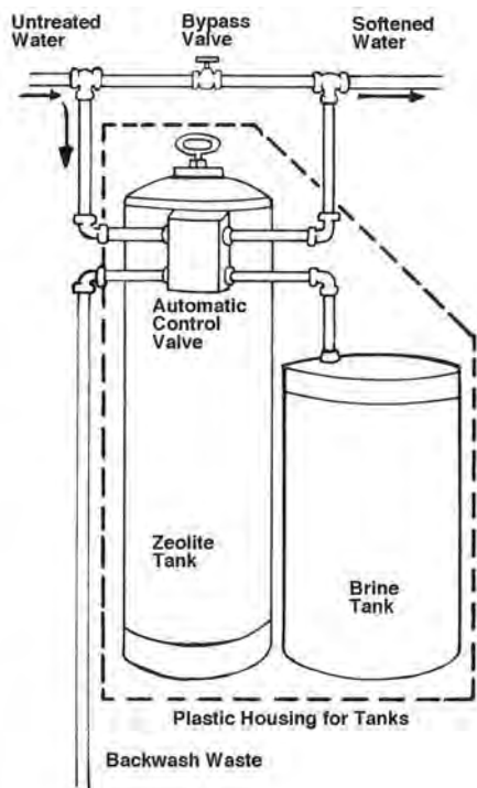
Figure 2. Automatic water softener – two tanks.
